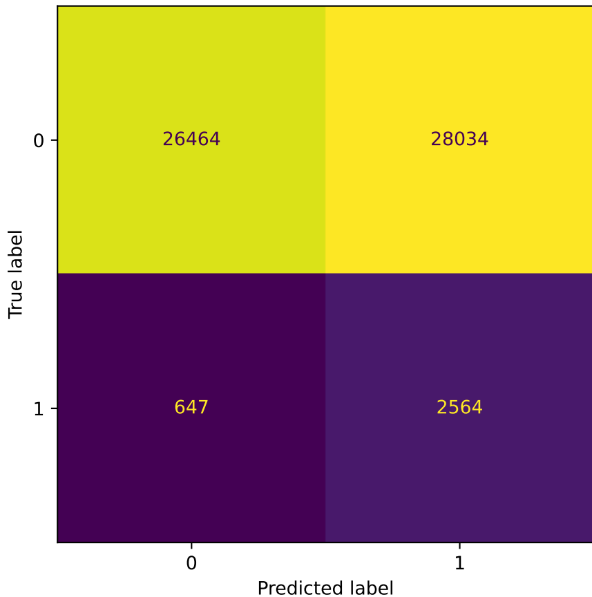
EXP-7 [abstracted] holdout confusion matrix (threshold=0)
