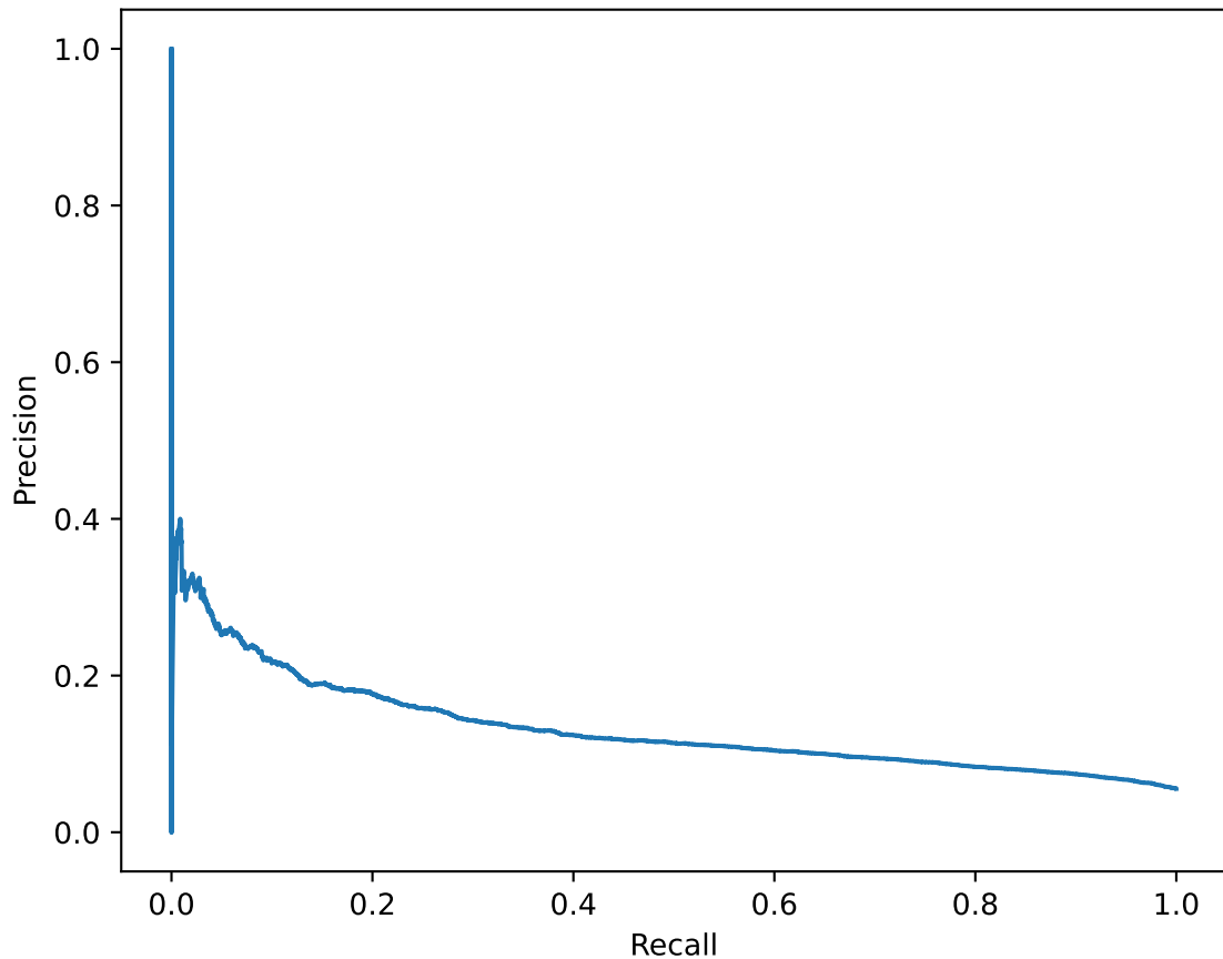
EXP-7 [abstracted] holdout PR curve (PR-AUC=0.1321)
