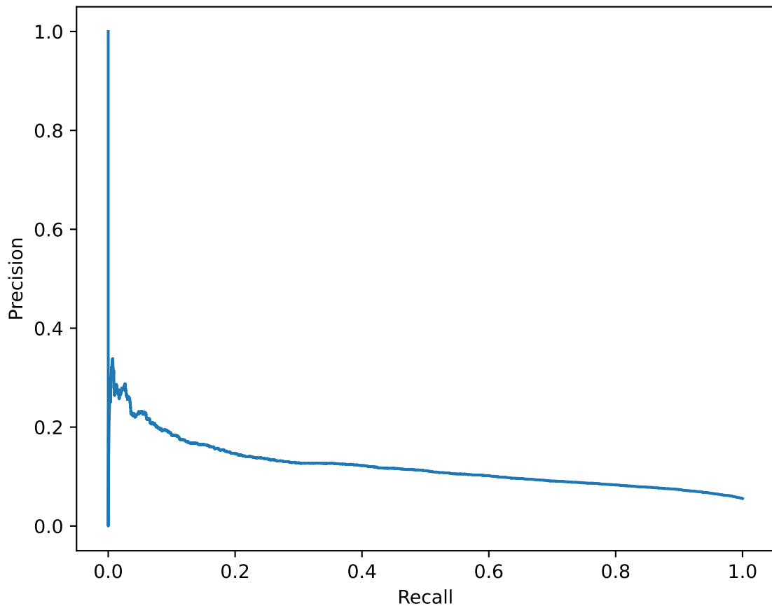
EXP-7 [normalized] holdout PR curve (PR-AUC=0.1210)
