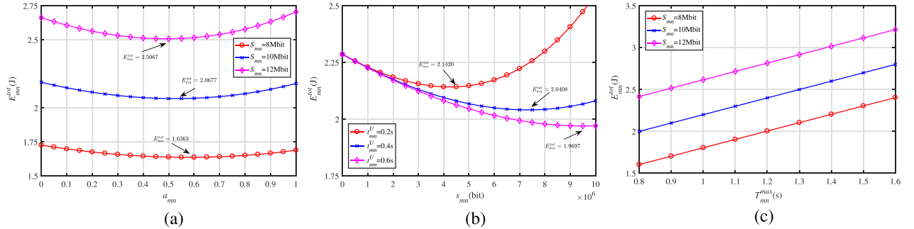
Fig. 7. The overall energy consumption under different values of a_{mn} , s_{mn} and T_{mn}^{max} . (a) E_{mn}^{tot} vs. a_{mn} . (b) E_{mn}^{tot} vs. s_{mn} . (c) E_{mn}^{tot} vs. T_{mn}^{max} .
