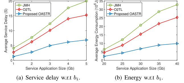
Fig. 10. Comparison on average service delay and energy with different b_i .
