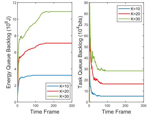
Fig. 6. Performance of queues backlog with different K .
