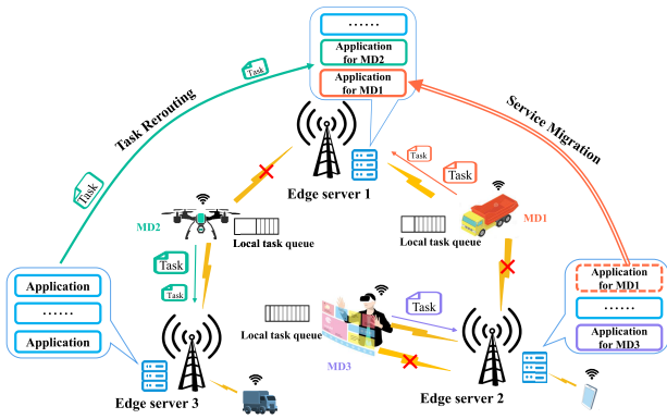
Fig. 1. An illustration of the considered system.
