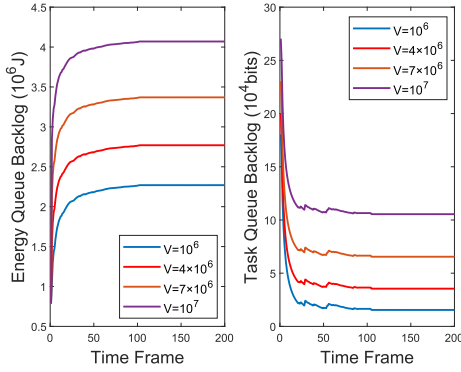
Fig. 5. Performance of queues backlog with different V .
