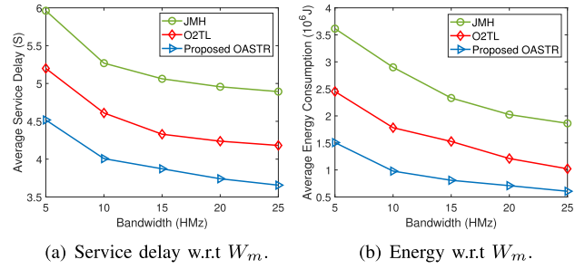
Fig. 7. Comparison on average service delay and energy consumption with different bandwidth.
