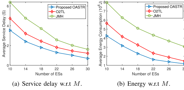
Fig. 8. Comparison on average service delay and energy with different number of ESs.
