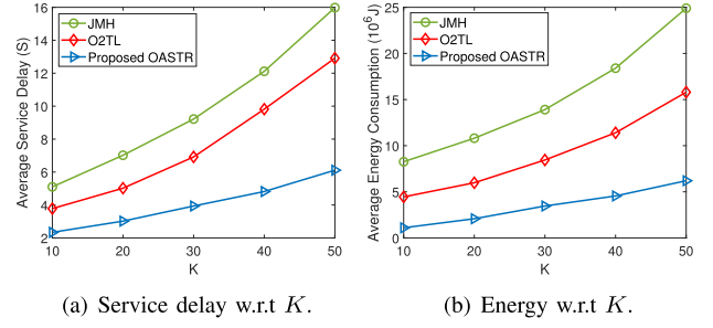
Fig. 9. Comparison on average service delay and energy with different K in each frame.
