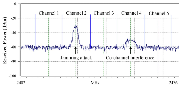
Fig. 10. Spectrum of five channels under jammer attacks.
