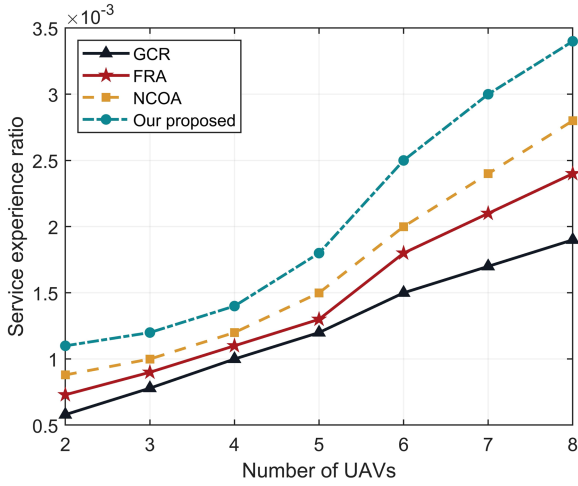
Fig. 5. Service experience ratio with different number of UAVs.
