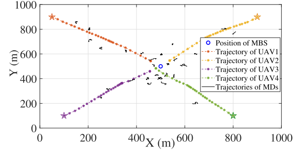
Fig. 4. Trajectories of the MDs and UAVs.
