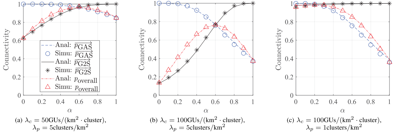
Fig. 2. The overall path connectivity metric ( p_{\text{overall}} ) versus \alpha , where \{\eta_x, \eta_y\} = \{0.1, 0.1\} , \{m_1, m_2, m_3\} = \{5, 5, 5\} , \{N_1, N_2, N_3\} = \{5, 10, 10\} , \{\gamma_1, \gamma_2, \gamma_3\} = \{0, -10, -10\} dB, \{f_1, f_2, f_3\} = \{0.9, 20, 20\} GHz, and H_s = 600 km.
