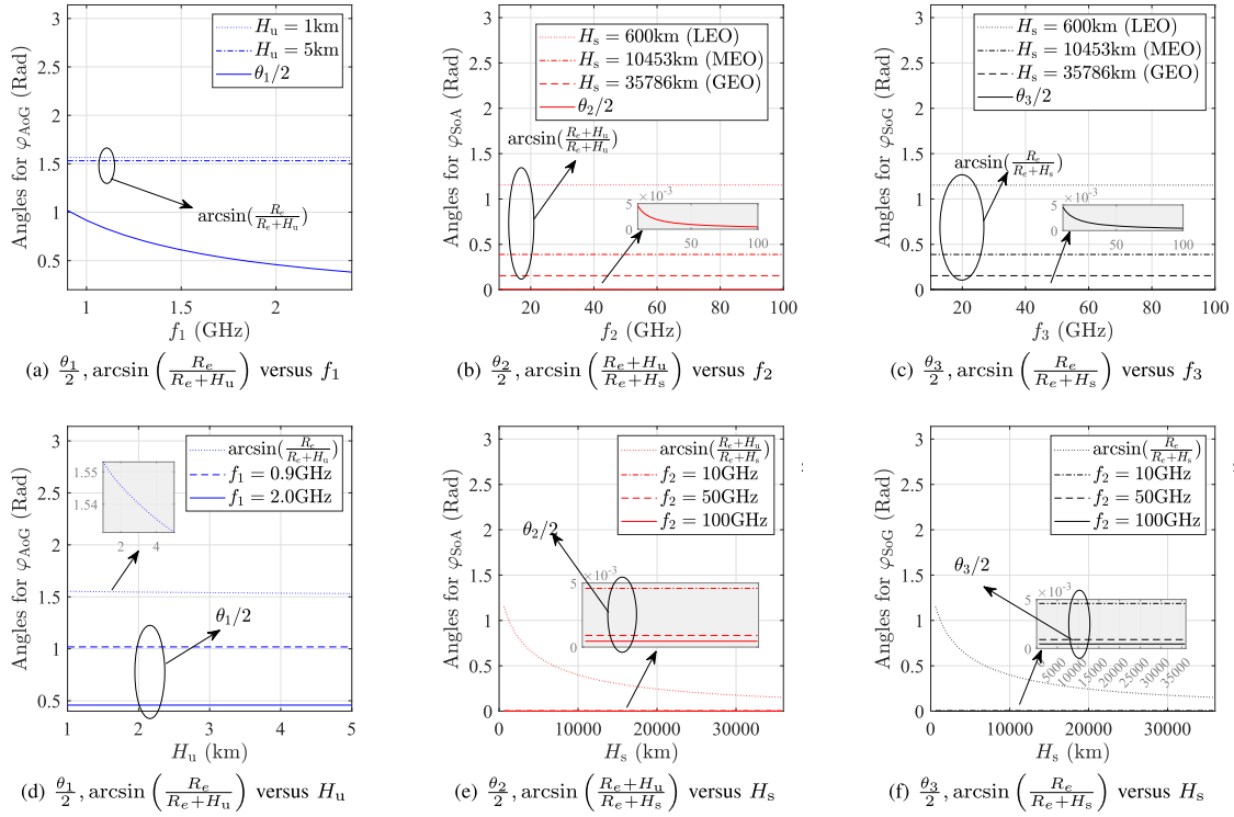
Fig. 6. Six angles (i.e., \theta_1/2, \theta_2/2, \theta_3/2, \arcsin(R_e/(R_e + H_u)) , \arcsin(R_e + H_u/(R_e + H_s)) , and \arcsin(R_e/(R_e + H_s)) ) versus carrier frequencies and the AV height/the satellite altitude. Herein, all system parameters (e.g., \kappa_i, D_i, \nu_i, \forall i \in \{1, 2, 3\} ) are set according to Table I.
