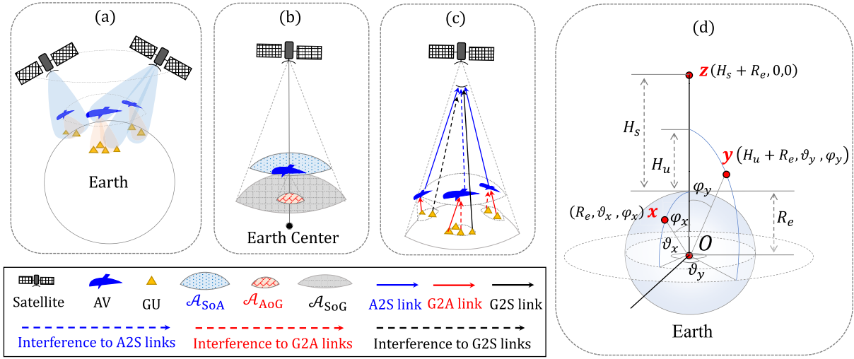
Fig. 1. Network Model of a SAGIN, where (a) is a SAGIN network, (b) shows three spherical coverage regions, (c) shows three transmission links, and (d) is the spherical coordinate system. Herein, \mathcal{A}_{AoG} , \mathcal{A}_{SoA} , and \mathcal{A}_{SoG} denote the coverage regions of the AV on the ground, the satellite on the AV-flying plane, and the satellite on the ground, respectively.
