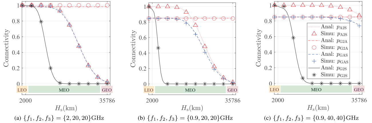
Fig. 4. Four connectivity metrics (i.e., p_{G2A} , p_{A2S} , p_{GAS} , and p_{G2S} ) versus H_s and f_i , where \lambda_c = 50 GU/(km 2 · cluster), \lambda_p = 0.1 clusters/km 2 , \{\eta_x, \eta_y\} = \{0.1, 0.1\} , \{m_1, m_2, m_3\} = \{5, 5, 5\} , \{N_1, N_2, N_3\} = \{5, 10, 10\} , \{\gamma_1, \gamma_2, \gamma_3\} = \{0, -10, -10\} dB, and H_u = 1000 m. Herein, LEO, MEO, and GEO represent three satellite orbits with varying altitudes, i.e., H_s \leq 2000 km, 2000 \text{ km} \leq H_s \leq 35786 km, and H_s = 35786 km, respectively.
