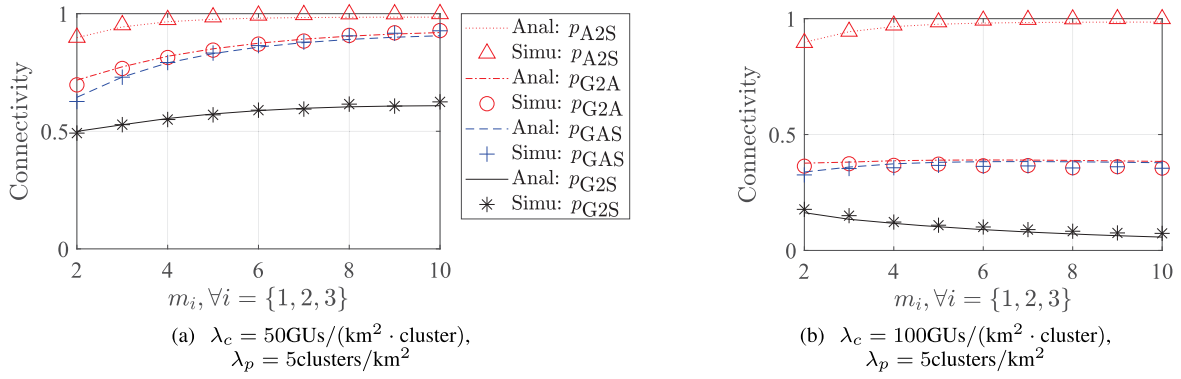
Fig. 3. Four connectivity metrics (i.e., p_{G2A} , p_{A2S} , p_{GAS} , and p_{G2S} ) versus m_i (\forall i \in \{1, 2, 3\}) , where \{\eta_x, \eta_y\} = \{0.1, 0.9\} , \{N_1, N_2, N_3\} = \{5, 10, 10\} , \{\gamma_1, \gamma_2, \gamma_3\} = \{0, -10, -10\} dB, \{f_1, f_2, f_3\} = \{0.9, 20, 20\} GHz, and H_s = 600 km.
