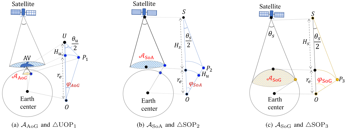
Fig. 5. Geometry relationship in coverage regions, where S is the satellite, O is the earth center, U is the AV, and P_1, P_2, P_3 are the points at the edge of \mathcal{A}_{AoG} , \mathcal{A}_{SoA} , and \mathcal{A}_{SoG} , respectively.
