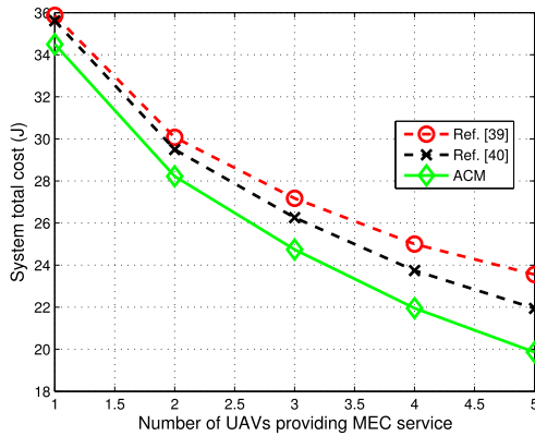
(b) Comparison for variable number of UAVs.
