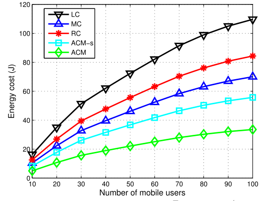
(a) Total cost in joules with \sigma_k^E = 1 and \sigma_k^\psi = 0 .
