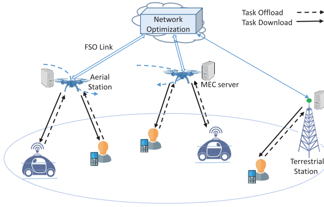
Fig. 1. Schematic diagram of the MEC-assisted multi-UAV aerial-terrestrial network.
