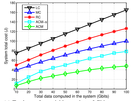
(a) Total cost for variable number of Gbits computed.
