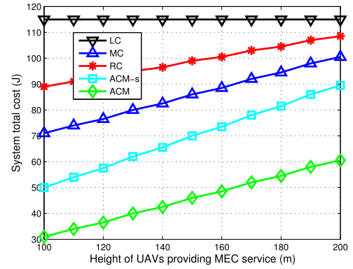
(c) Total cost for variable height of UAVs.
