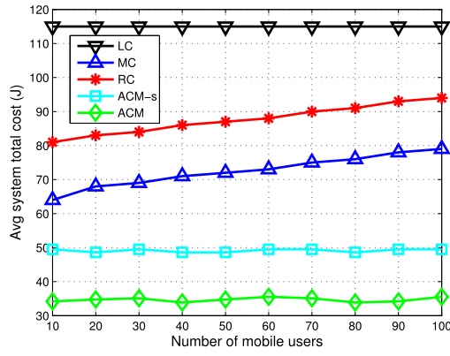
(a) Average system total cost.
