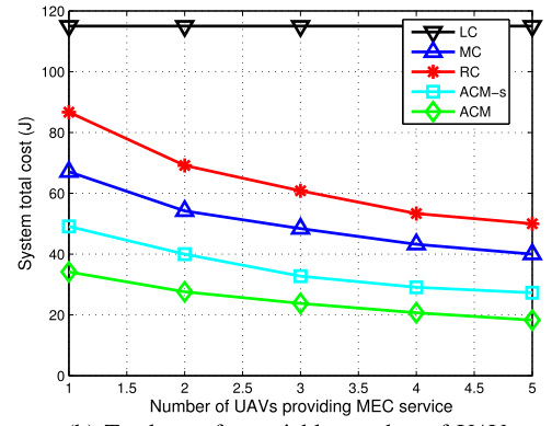
(b) Total cost for variable number of UAVs.
