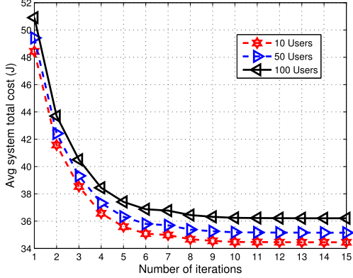
(b) Convergence of the proposed joint optimization.
