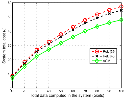
(a) Comparison for variable number of Gbits computed.
