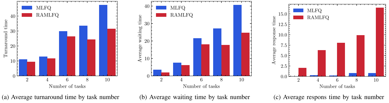
Fig. 13. The performance of computing resource allocation based on CPU task scheduling.
