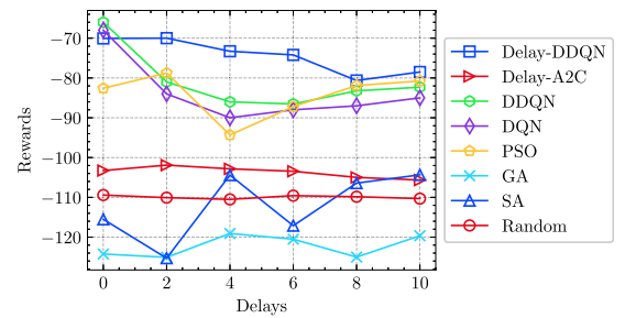
Fig. 6. Comparison of different algorithms under fixed state delays.
