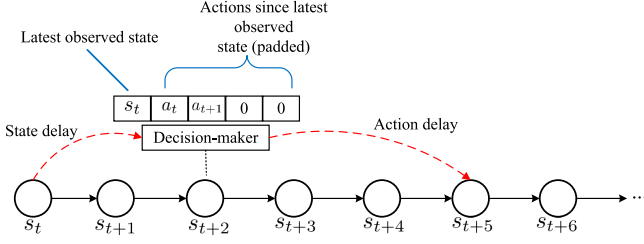
Fig. 3. Graphical illustration of the problem of the LEO satellite-terrestrial integrated networks with system state delay.
