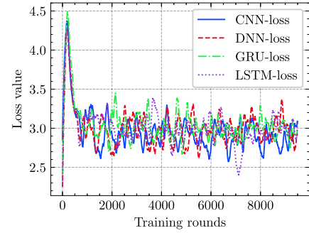
Fig. 10. Comparisons with neural networks for loss value.
