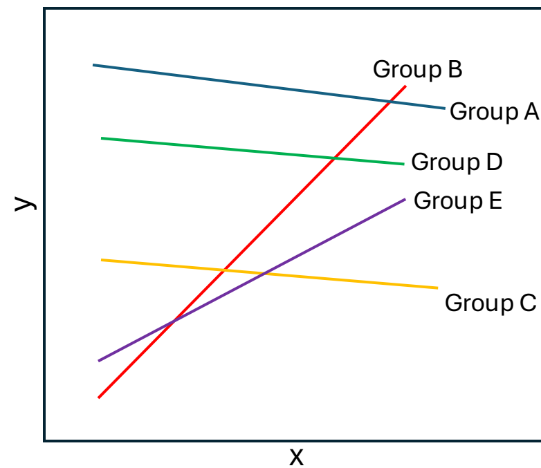
Random Intercepts and Slopes
