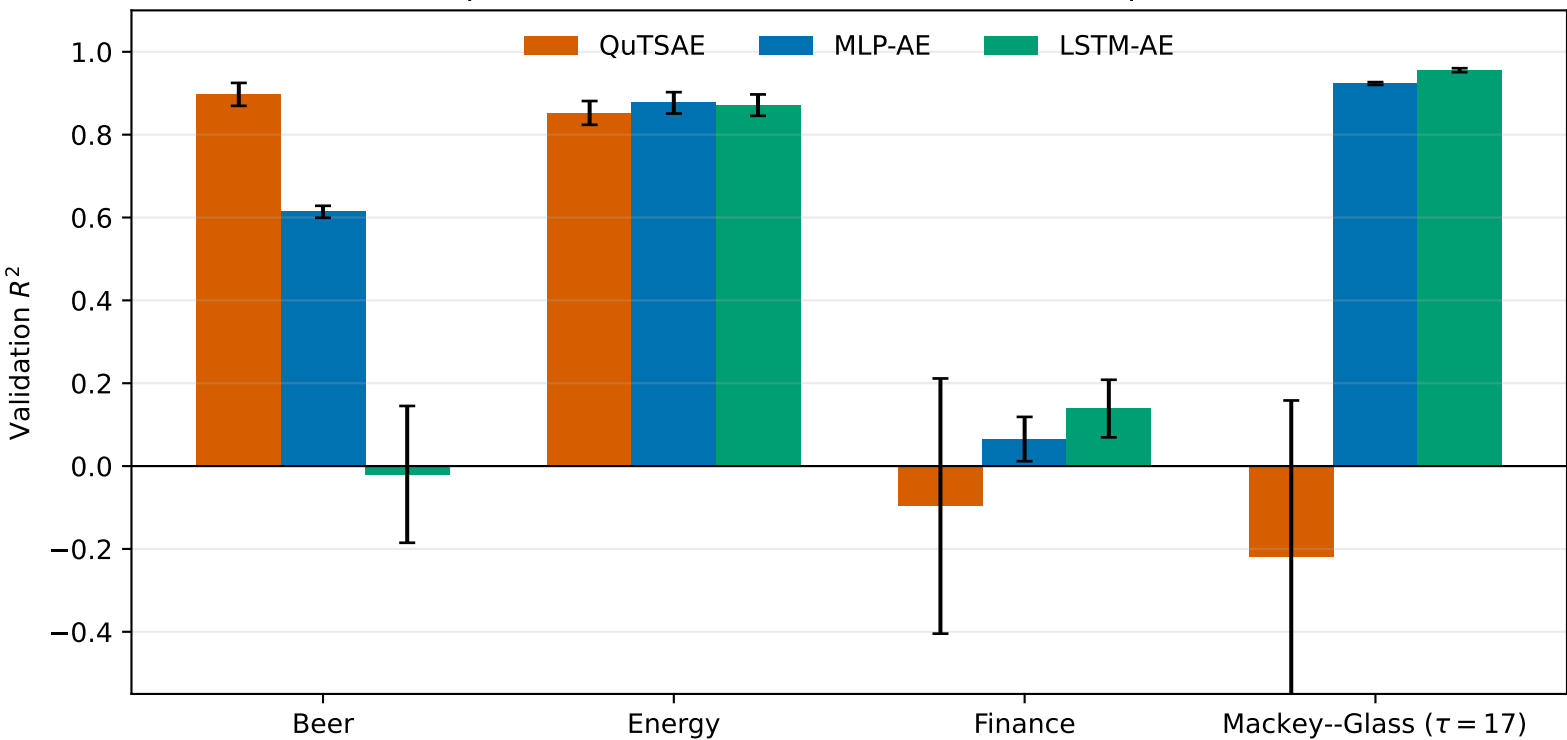
Independent Qiskit/Aer validation (five seeds per model)
