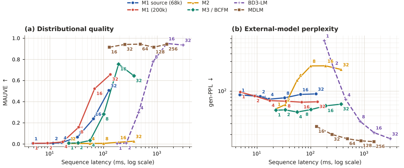
Figure 1. TinyStories quality versus batch-one sequence latency on one H100 NVL. Numbers next to points are NFE. Solid curves use argmax CFM-family endpoints; dashed curves use the canonical stochastic MDLM/BD3-LM samplers. All points use the same 512-sample quality protocol and the same batch-one FP32 latency protocol.
