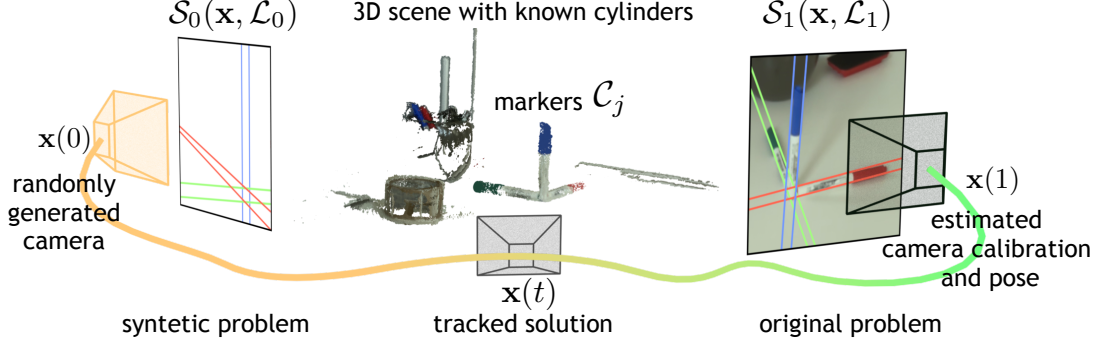
Figure 1: Our method for N = 1 camera and M = 3 cylindrical objects (3 markers). The input is a known 3D scene and images with estimated silhouette lines. The output is the calibration and the pose of the cameras that acquired the images. Rather than tackling the problem on the input data, we move to a simpler random problem with a known solution \mathbf{x}(0) . Our silhouette-based parametric homotopy allows to track \mathbf{x}(0) to the solution \mathbf{x}(1) of the original problem. Our formulation support multiple cylinders and multiple images.
