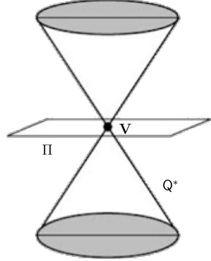
(b) An example of a plane \Pi tangent to a cone C , which does not define the quadric surface Q^*
