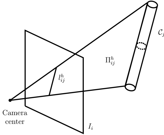
Figure 2: The geometric constraints between a cylinder C_j and one of its silhouette lines l_{ij}^h . The backprojection of l_{ij}^h is a plane \Pi_{ij}^h tangent to C_{ij} (??) and passing to the point at infinity of the cylinder(??), i.e. , parallel to its axis.
