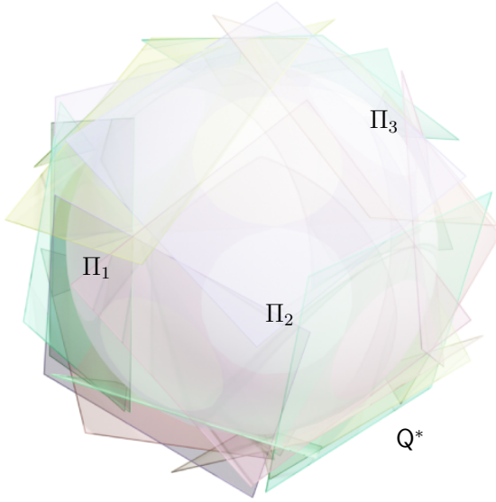
(a) The plane envelop of a dual quadric Q^* . Tangent planes \Pi_i define the overall surface
