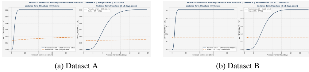
Figure 6: Variance term structure, both datasets: the piecewise-constant- h CAR(4) approximation of Tol [1997] against the simplified Heston/CIR CAR(1) term structure of Section 5.6. Left panel of each pair: full term structure, 0–90 days, showing convergence of the two approximations at long horizons. Right panel: zoomed view, 0–14 days, isolating the short-horizon divergence driven by the CAR(4) kernel’s g(0) = 0 property.
