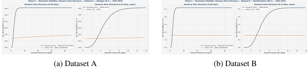
Figure 6: Variance term structure, both datasets: the piecewise-constant- h CAR(4) approximation of Tol [1997] against the simplified Heston/CIR CAR(1) term structure of Section 5.6. Each panel contains two plots, side by side. Left: the full term structure over a 0–90-day horizon, showing the two approximations converging at long horizons. Right: a zoomed view over 0–14 days, isolating the short-horizon divergence driven by the CAR(4) kernel’s g(0) = 0 property.
