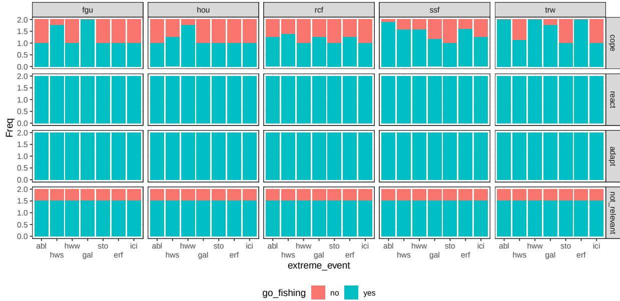
Figure B.10: conditional distribution for go_fishing . Columns represents levels of the node fishing_style ; rows are levels of the node strategy_to_change .
