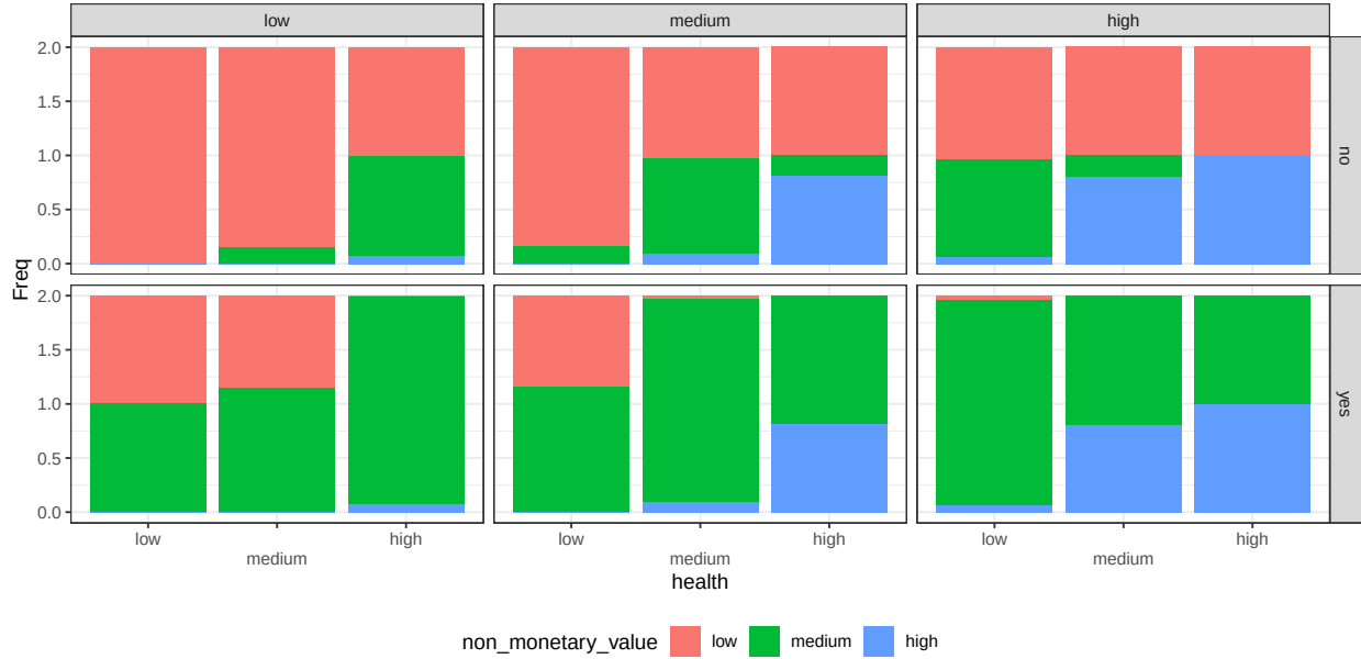
Figure B.15: conditional distribution for non_monetary_value. Columns represents levels of the node satisfaction; rows are levels of the node substitution_capacity.
