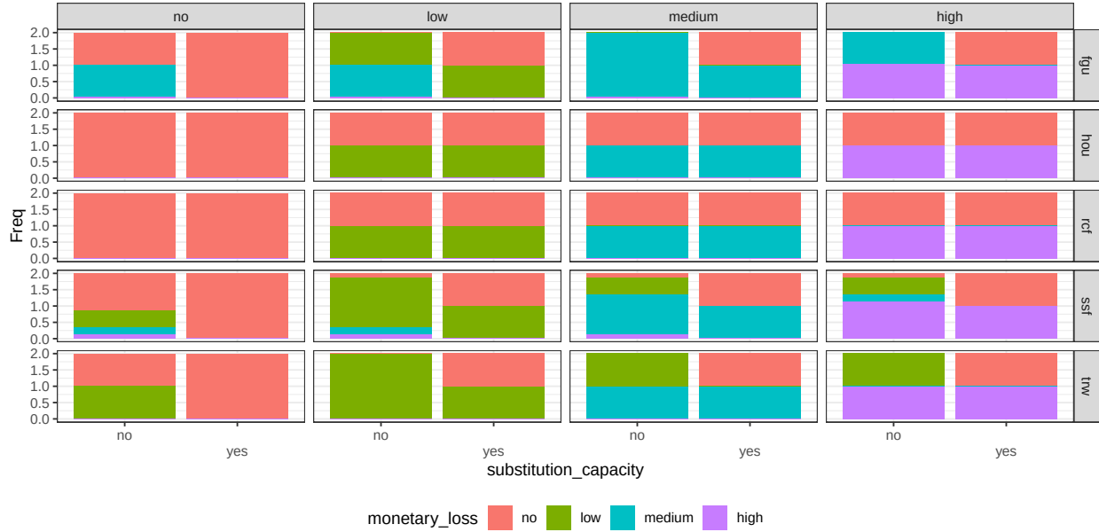
Figure B.17: conditional distribution for monetary_loss. Columns represents levels of the node costs; rows are levels of the node fishing_style.
