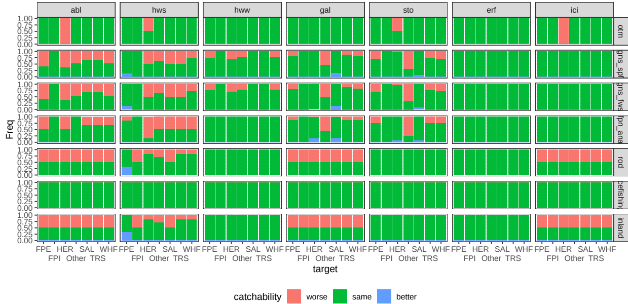
Figure B.5: conditional distribution for catchability. Columns represents levels of the node extreme_event; rows are levels of the node gear.
