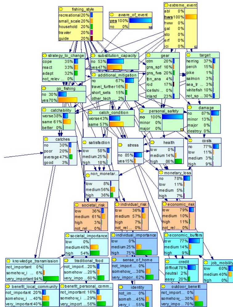
Figure B.1: complete representation of the Bayesian Network, showing conditional probabilities distributions. Colors are associated to node types and group Yellow: decision nodes; lime green: chance nodes - operational group; grey: chance nodes - user group; navy blue: chance nodes - individual group; light blue: chance nodes - societal group; cyan: chance nodes - economic group; orange: utility nodes - risk
