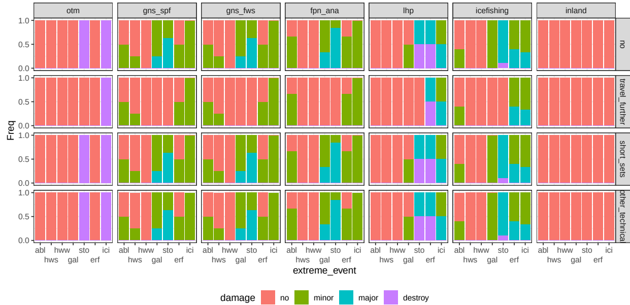
Figure B.8: conditional distribution for damage. Columns represents levels of the node gear; rows are levels of the node additional_mitigation.
