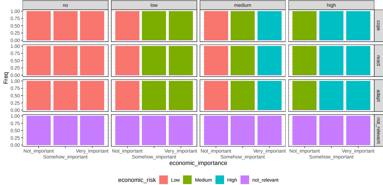
Figure B.34: conditional distribution for economic_risk. Columns represents levels of the node cost; rows are levels of the node strategy.
