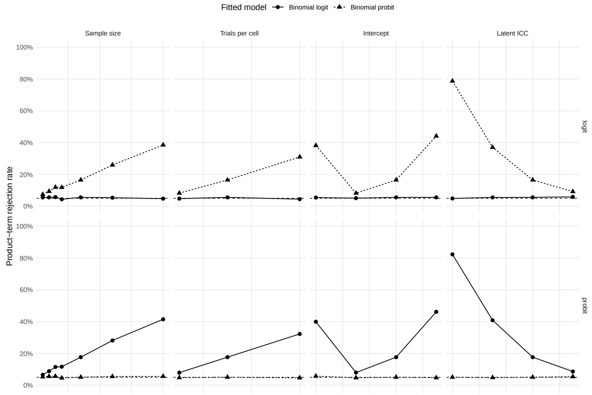
Figure 5: Logit-probit sensitivity slices. Rows identify the generating link. Within each panel the fitted logit and probit models are compared as one parameter varies around the manuscript anchor.
