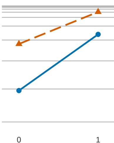
Standard logit B = +0.513
