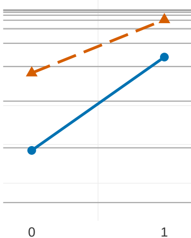
Standard logit B = +0.513
