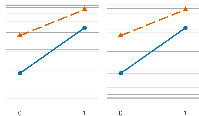
Standard logit B = +0.513
