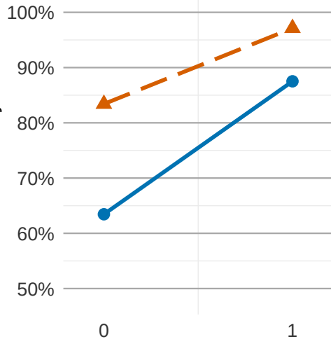
Linear (probability) B = -0.103
