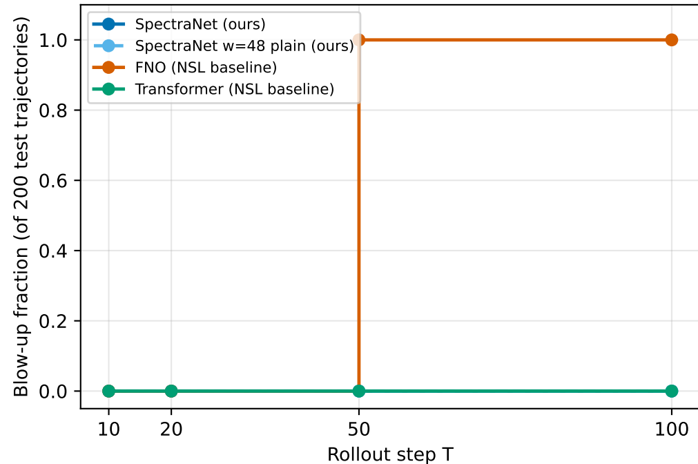
(a) Fraction of test trajectories that diverge by step T
