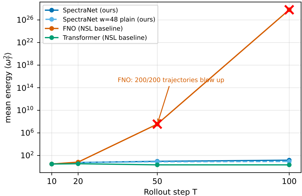
(b) Vorticity energy vs T (log-y) — FNO diverges at T \geq 50
