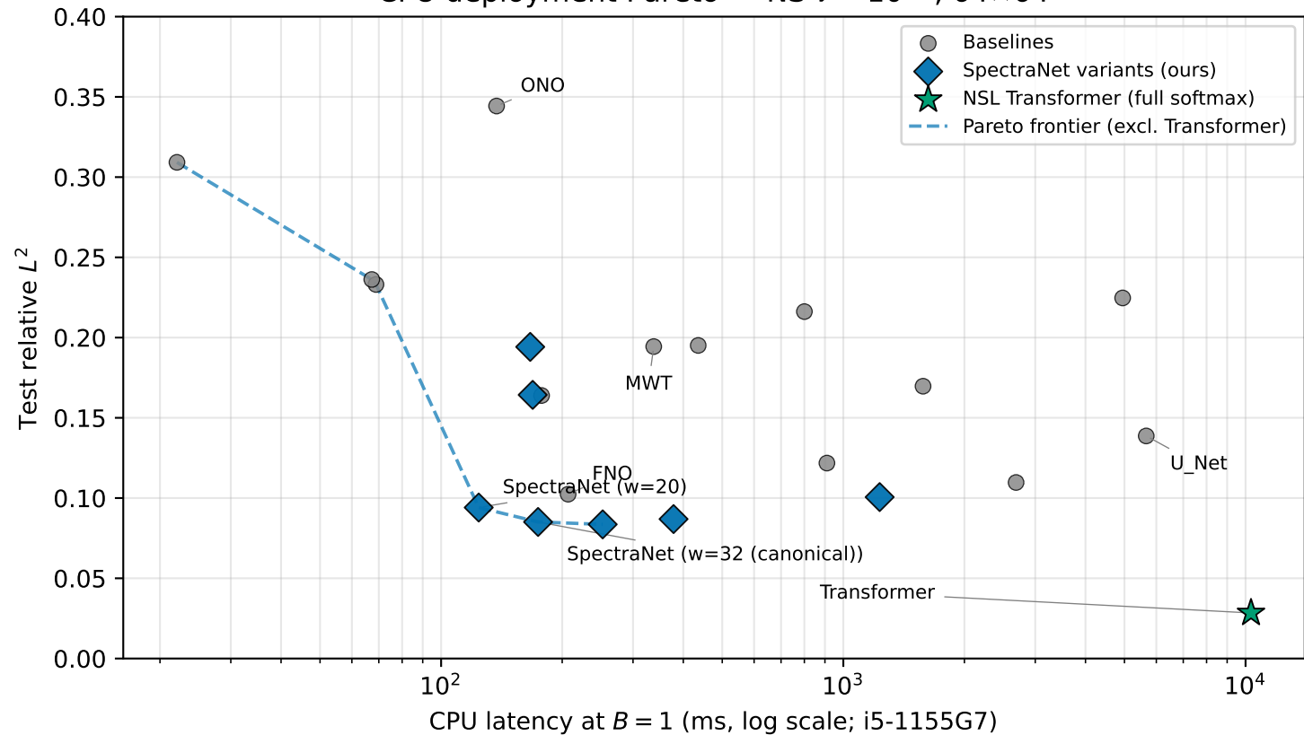
CPU deployment Pareto — NS \nu = 10^{-5} , 64 \times 64
