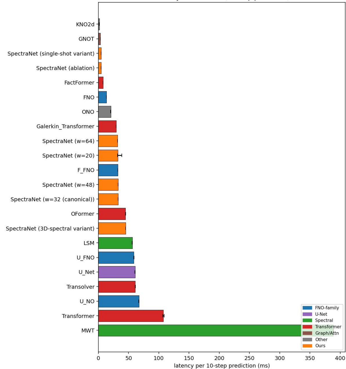
Latency — batch=1 (10-step prediction)
