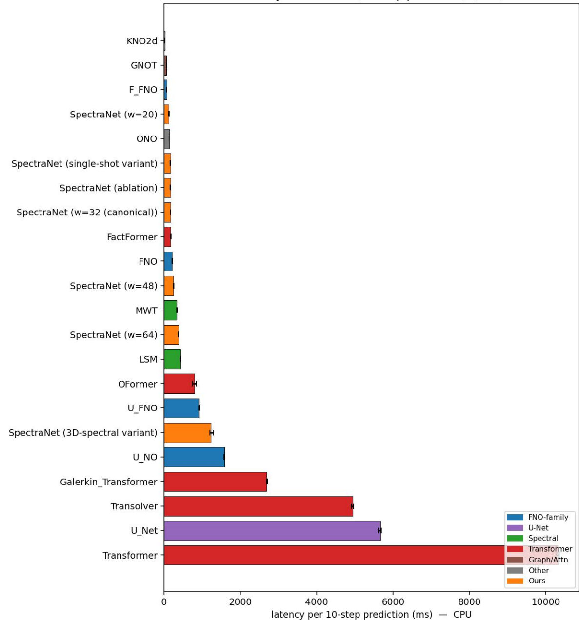
Latency — batch=1 (10-step prediction) (CPU)
