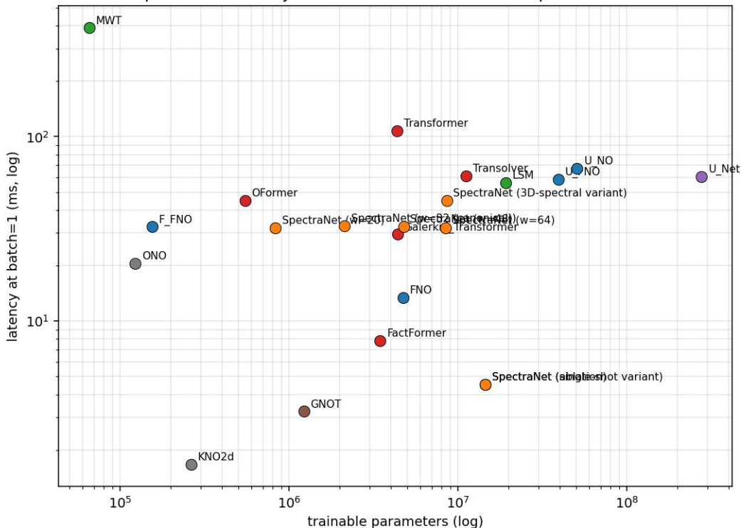
params vs latency — full attention is above the param-fit line
