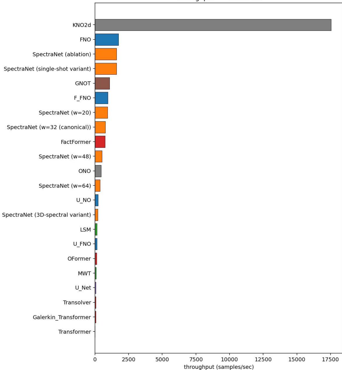
Throughput — batch=32
