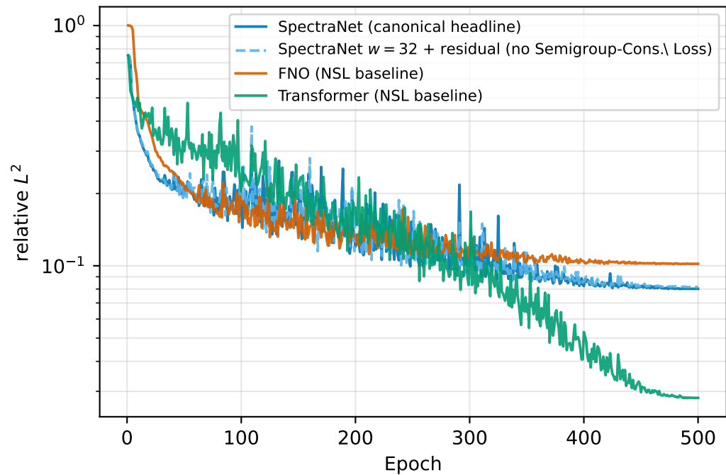
(b) Validation relative L^2
