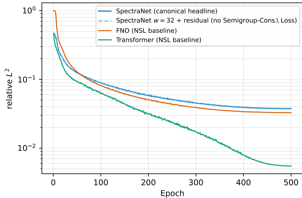
(a) Training relative L^2
