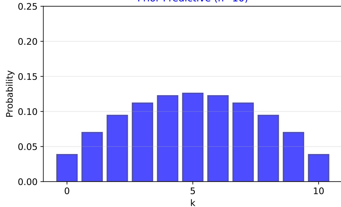
Prior Predictive (n=10)
