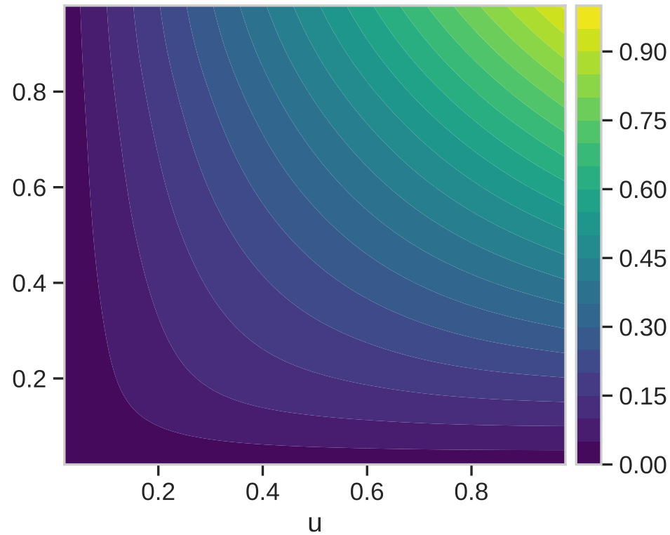
Bernstein approx. (degree=30)
