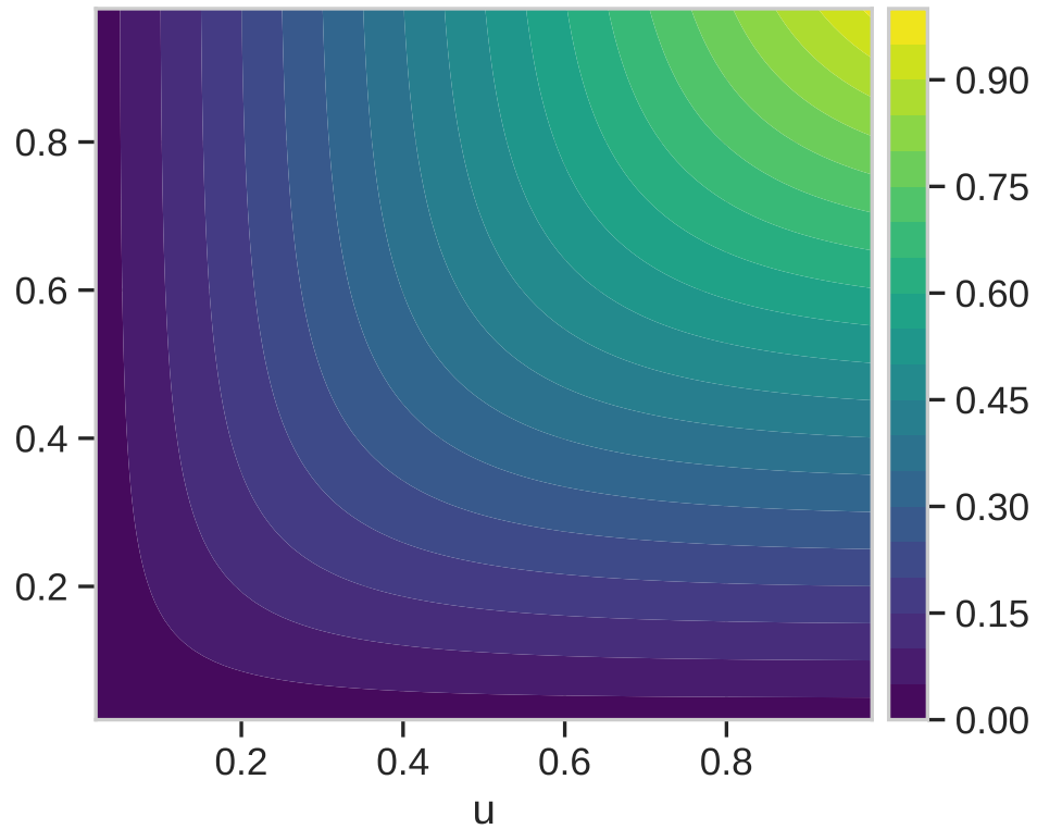
True Frank CDF ( \theta=5.00 )
