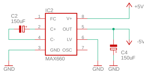
-5V supply
