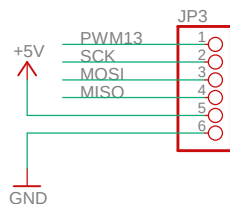
SD Card
