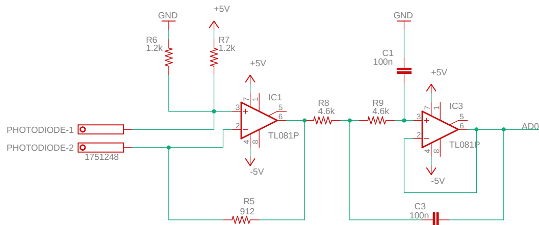
T2 Amplifier
