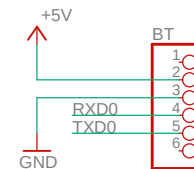
HC05 Bluetooth
