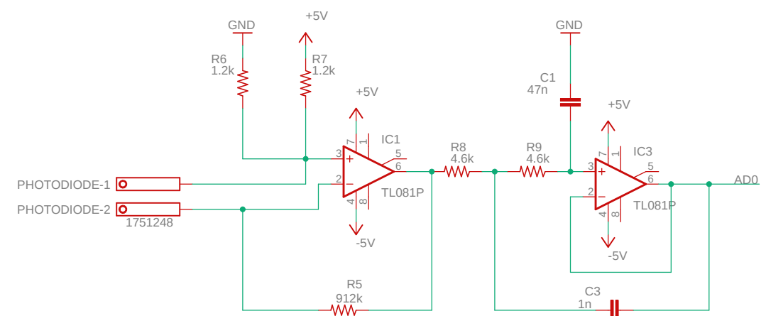
T2 Amplifier
