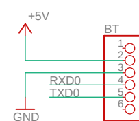
HC05 Bluetooth
