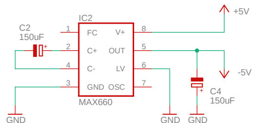
-5V supply
