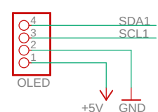
OLED I2C Screen
