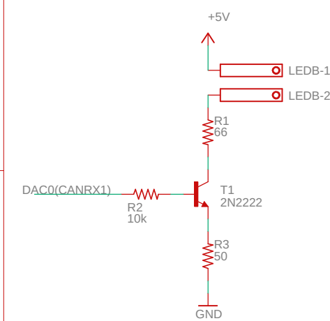
LED Power
