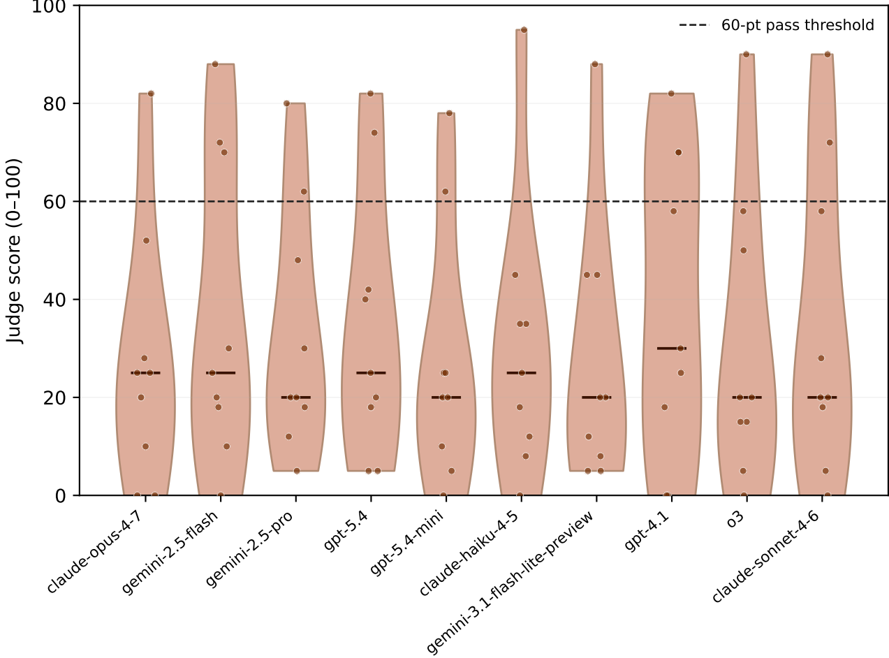
B. Open-ended judge-score distribution
