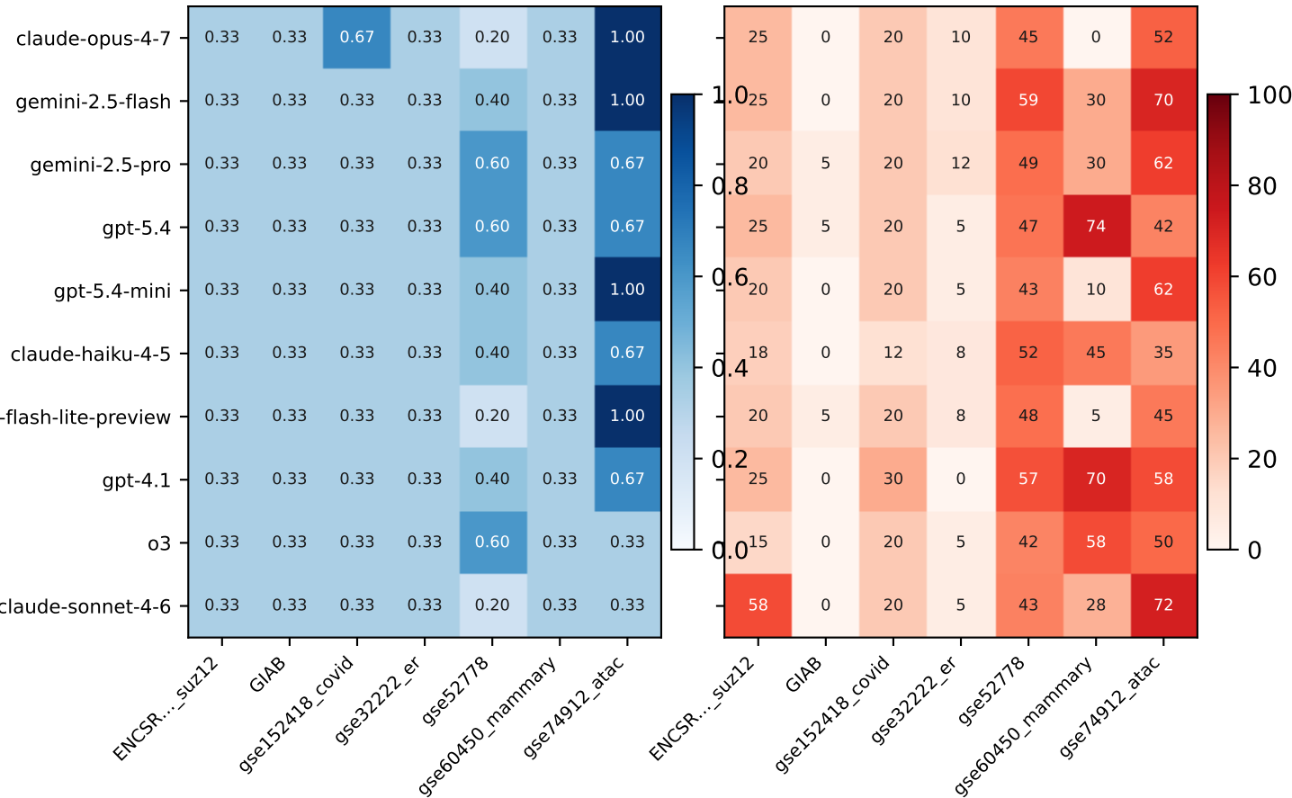
C. Per-dataset breakdown — MCQ and Open-ended mean judge score
