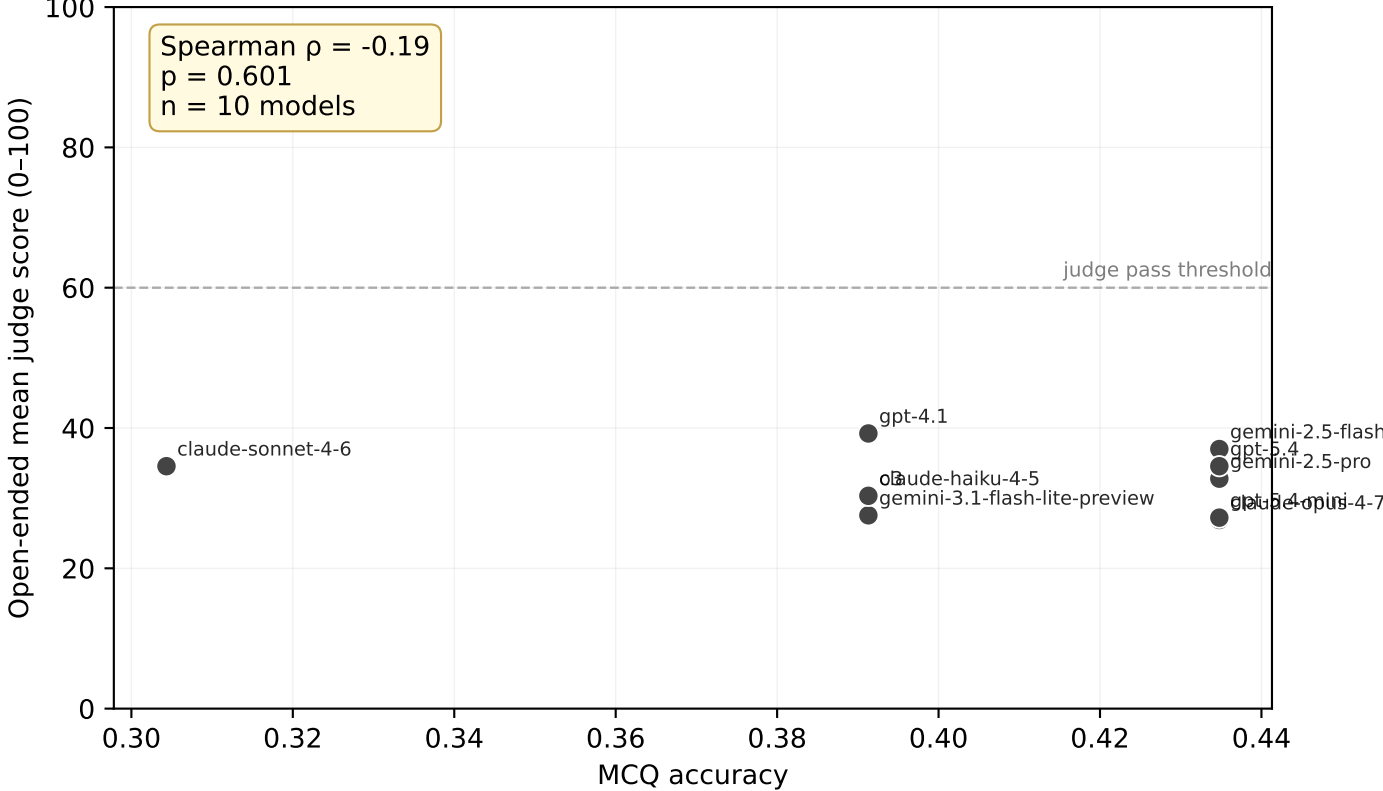
D. MCQ vs open-ended performance per model
