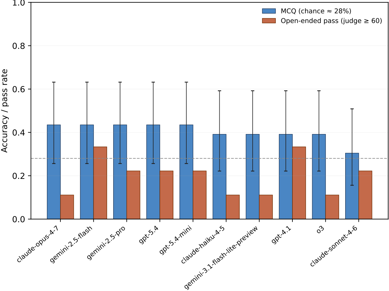
A. Per-model interpretation accuracy
