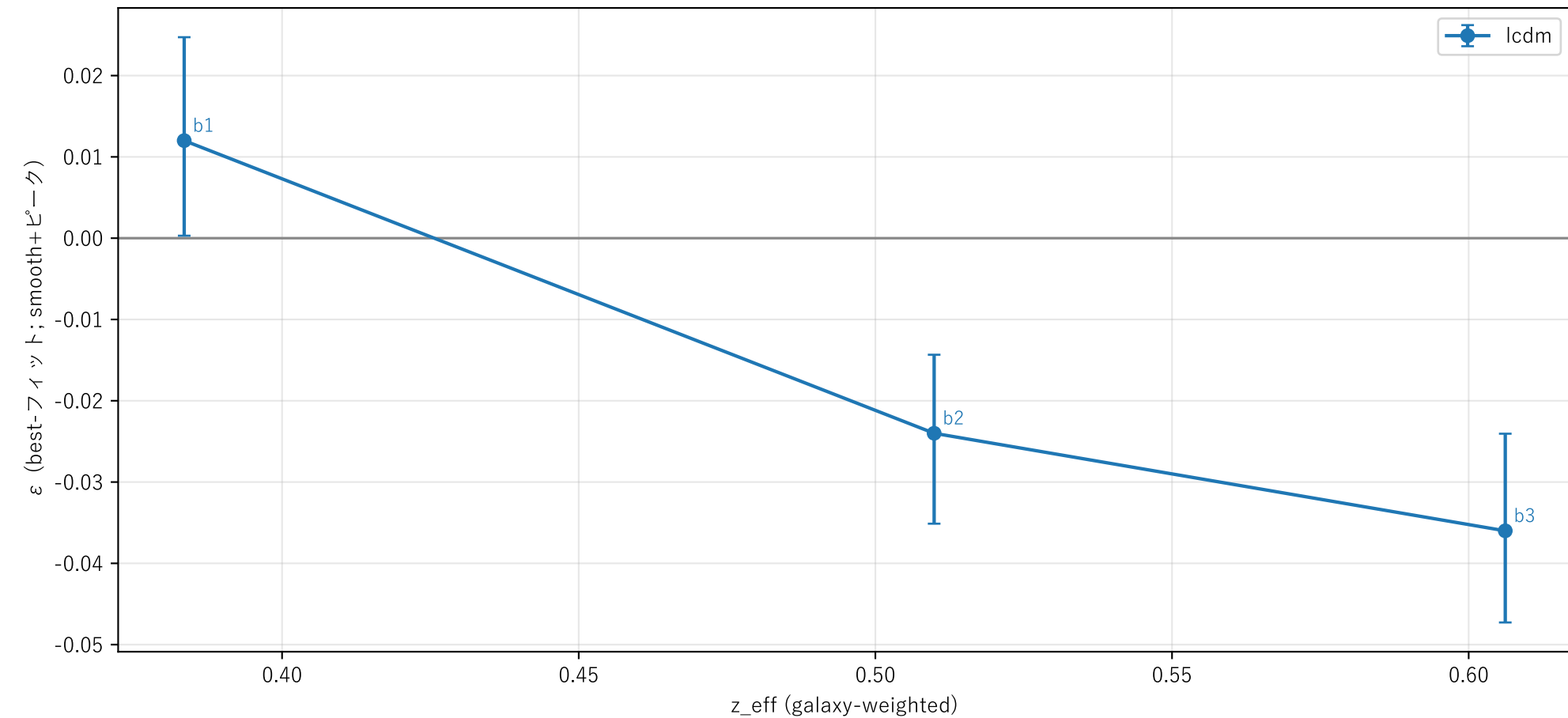
BAO catalog-based peakfit (cmasslowztot, combined) : \varepsilon(z) (smooth_p=2, cov=auto, quad_weight=1)
