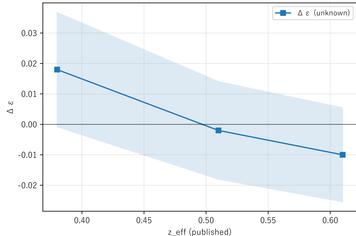
\Delta \varepsilon = \varepsilon_{\text{catalog}} - \varepsilon_{\text{published}} (\pm 1 \sigma \text{ sym})
