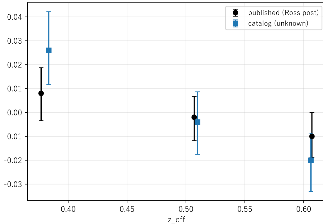
\varepsilon (AP warping) vs z
