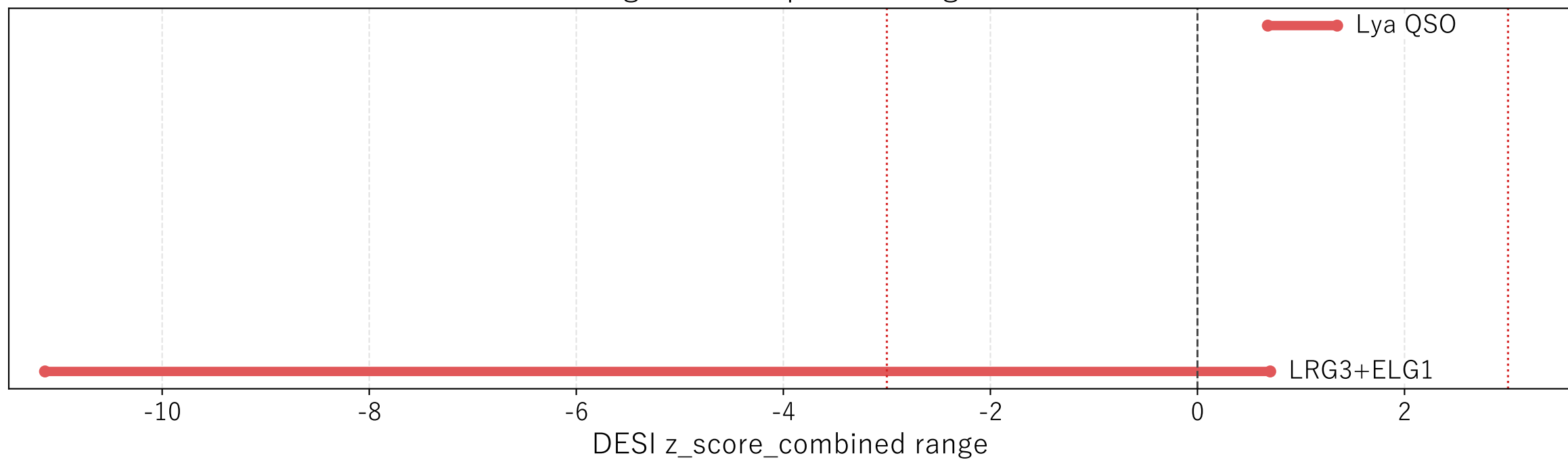
Stage B: DESI promotion gate
