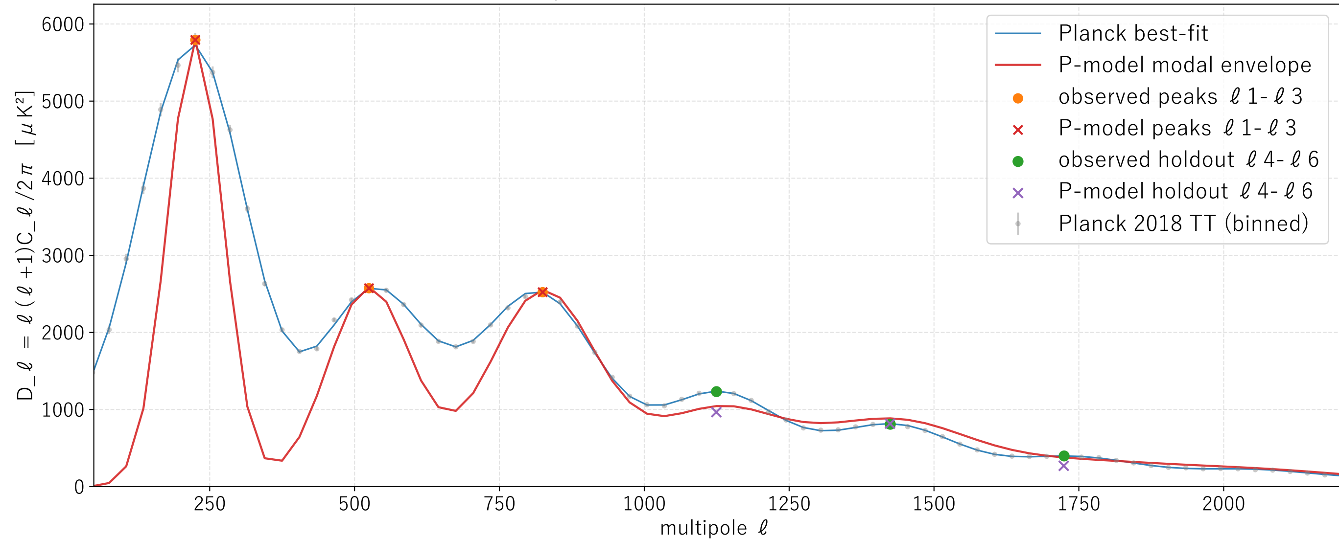
Peak residuals (first3 fit + \ell 4- \ell 6 holdout)
