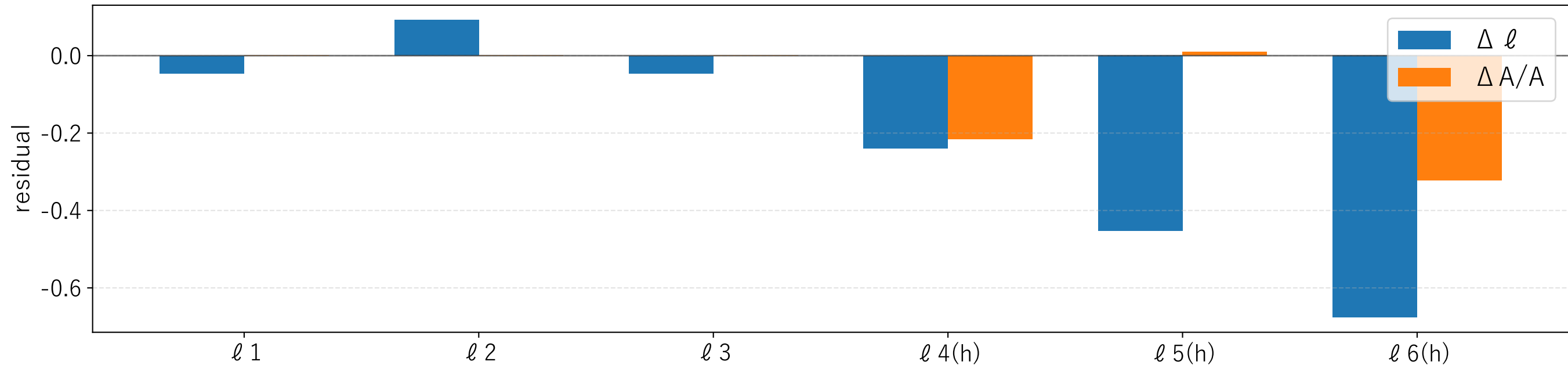
Peak residuals (first3 fit + \ell 4- \ell 6 holdout)
