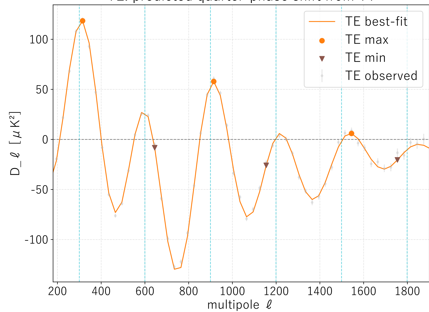
TE: predicted quarter-phase shift from TT
