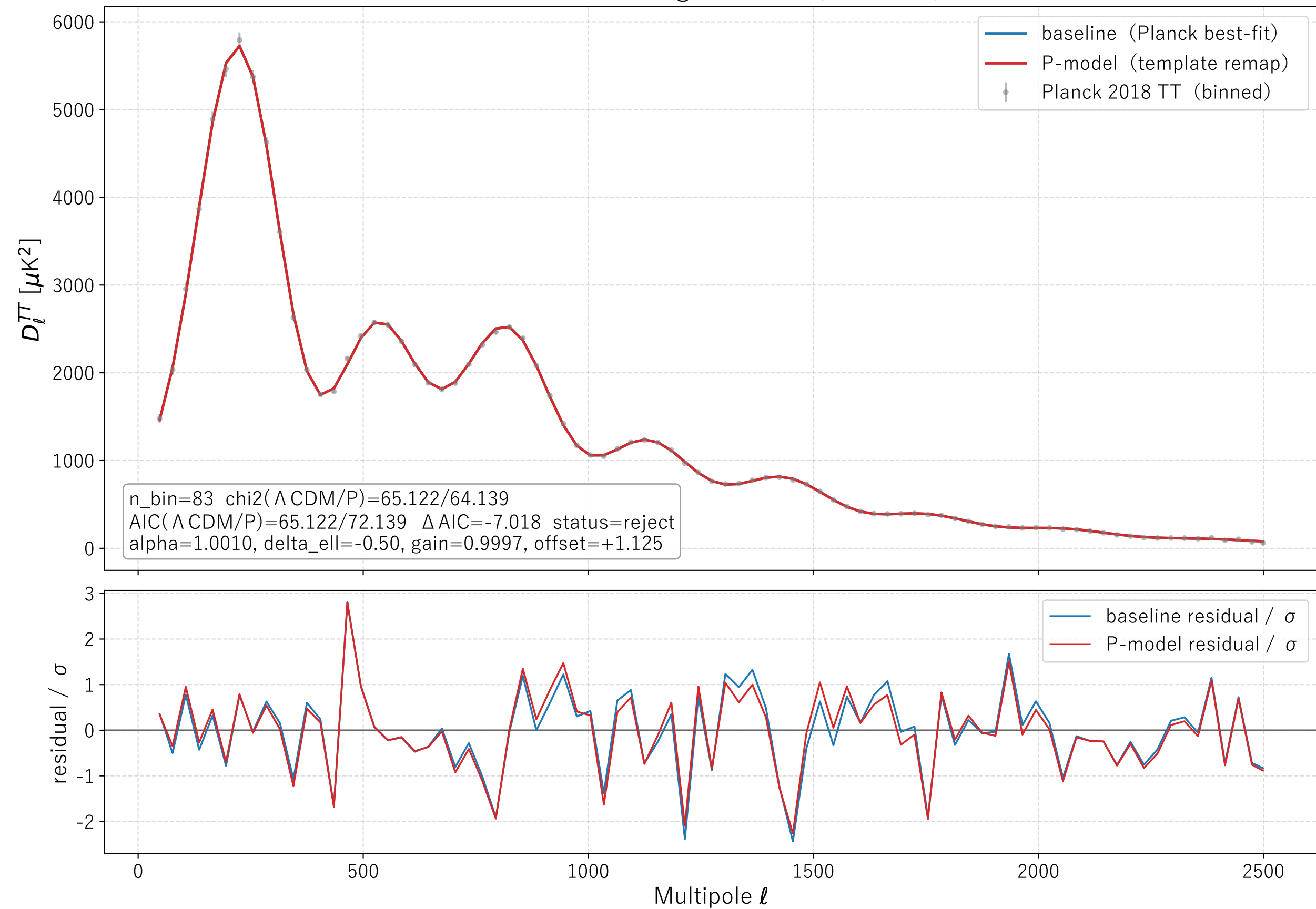
CMB TT full-range fit audit ( \ell \leq 2500 )
