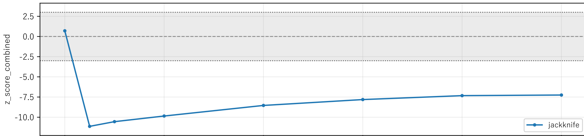
LRG3+ELG1 (dist=pbpg) z \in [-11.13, 0.70] stable( |z| \geq 3 )=no
