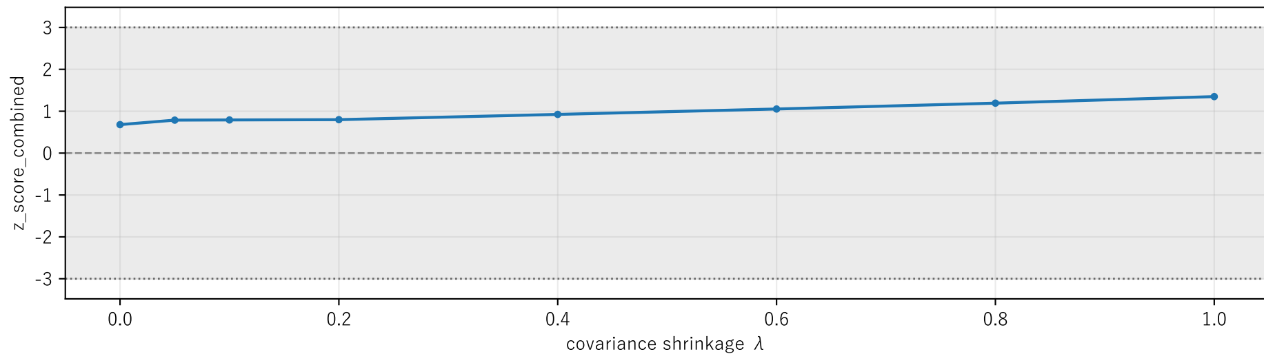
Lya QSO (dist=pbpg) z \in [0.68, 1.35] stable( |z| \geq 3 )=no
