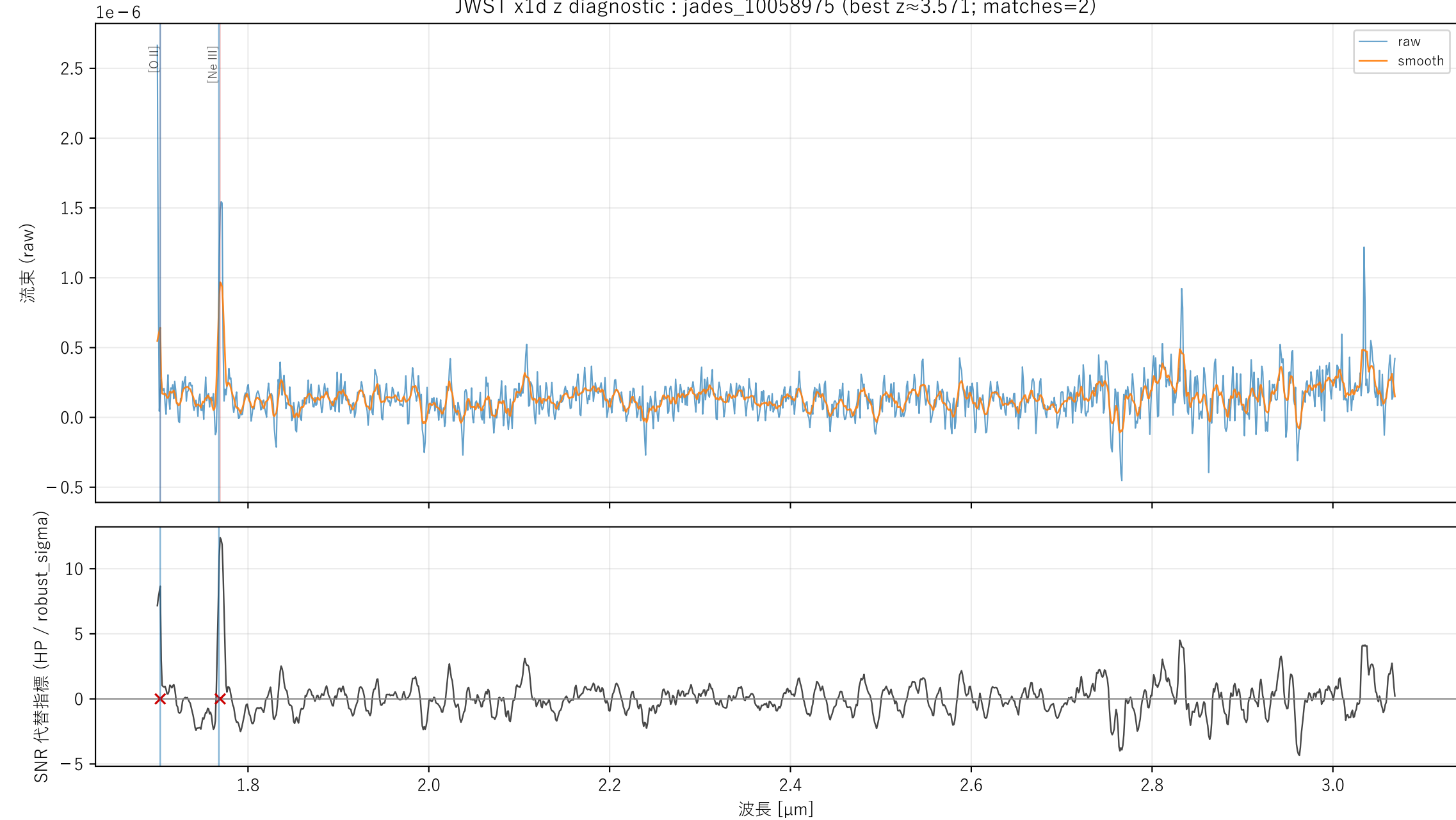
JWST x1d z diagnostic : jades_10058975 (best z \approx 3.571 ; matches=2)
