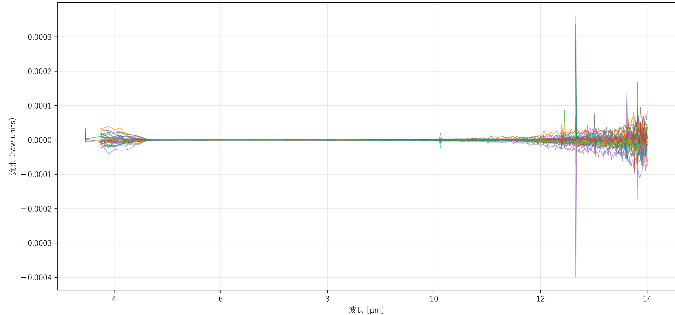
JWST x1d spectrum (MAST) : jades_gs_z14_0
