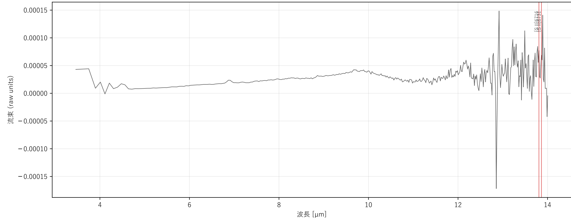
JWST x1d z confirmed : lid2619 ( z \approx 19.578 )
