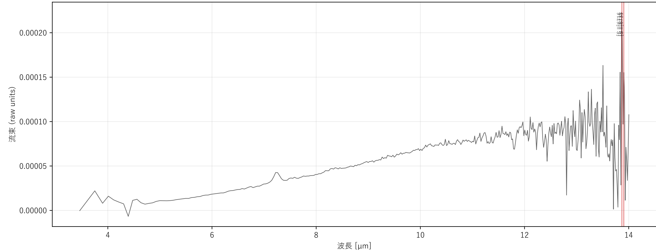
JWST x1d z confirmed : lid4959 ( z \approx 19.652 )
