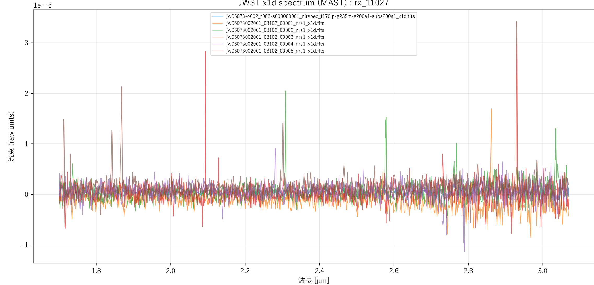
JWST x1d spectrum (MAST) : rx_11027
