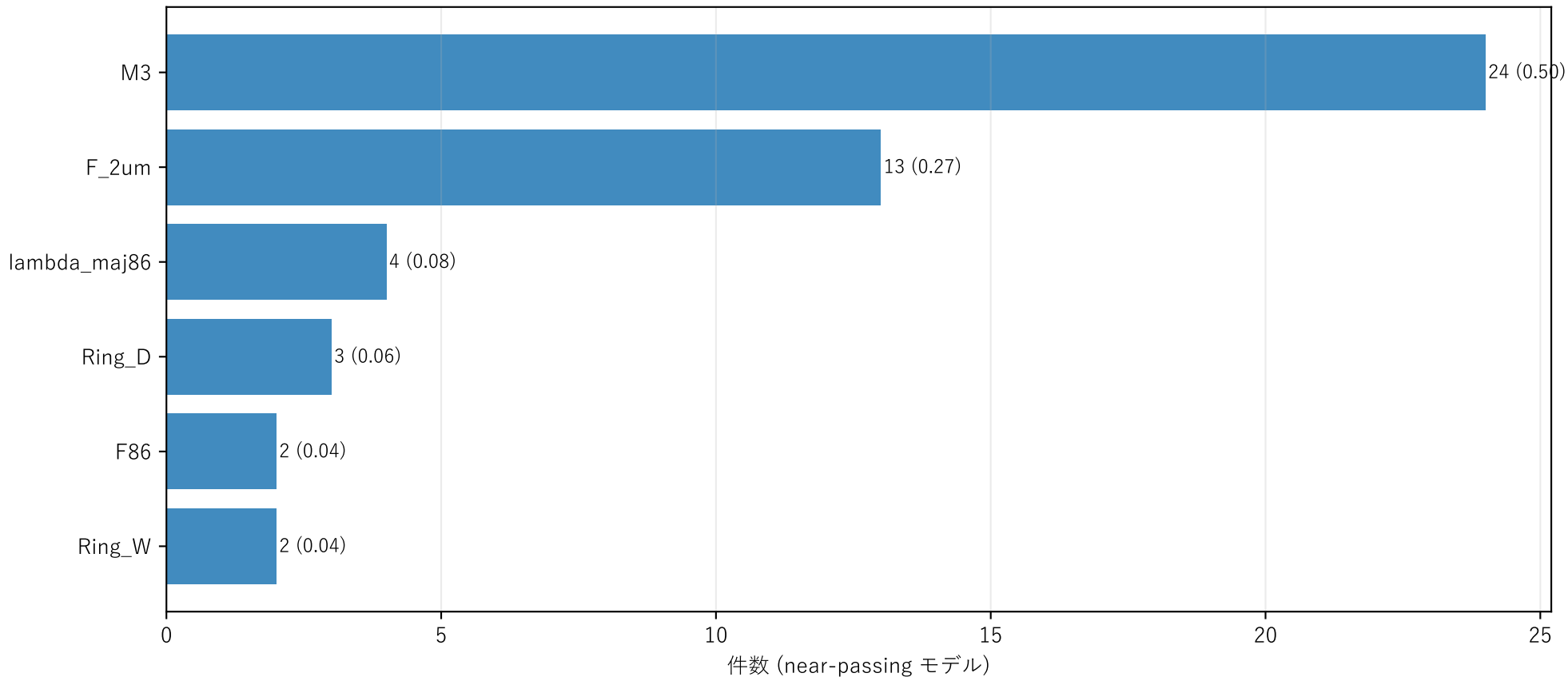
Paper V near-passing: failed constraint counts (fail_one + fail_none)
