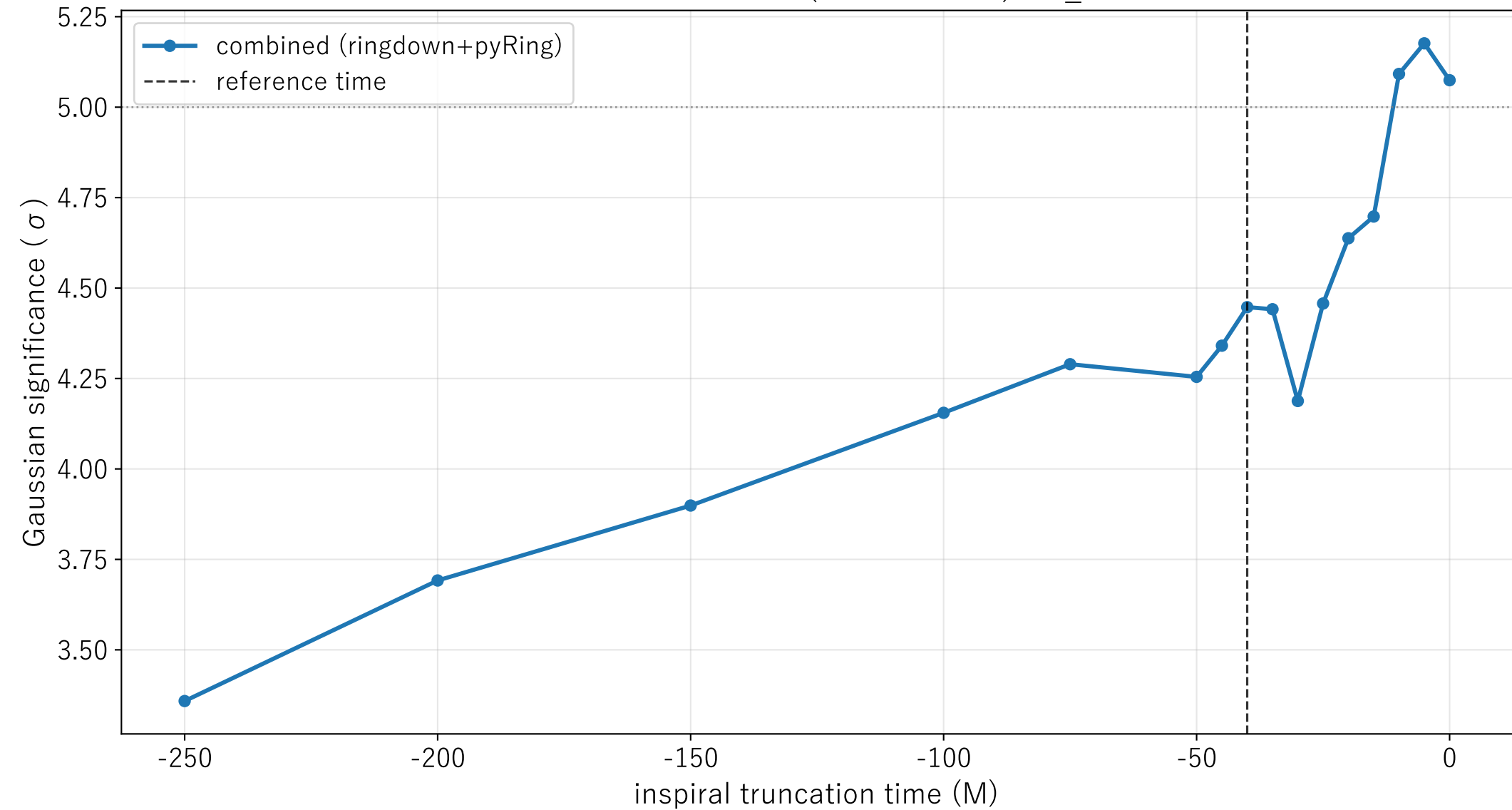
GW250114 area theorem (data release): \sigma_{\text{ref}}=4.45
