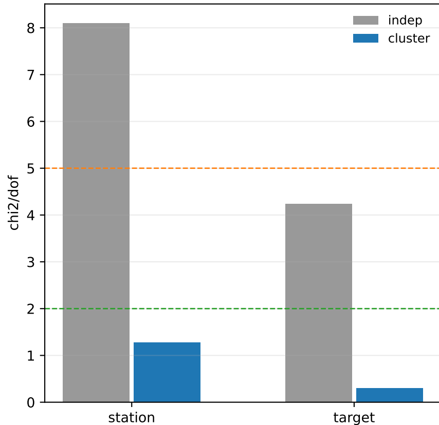
Stratified chi2/dof
